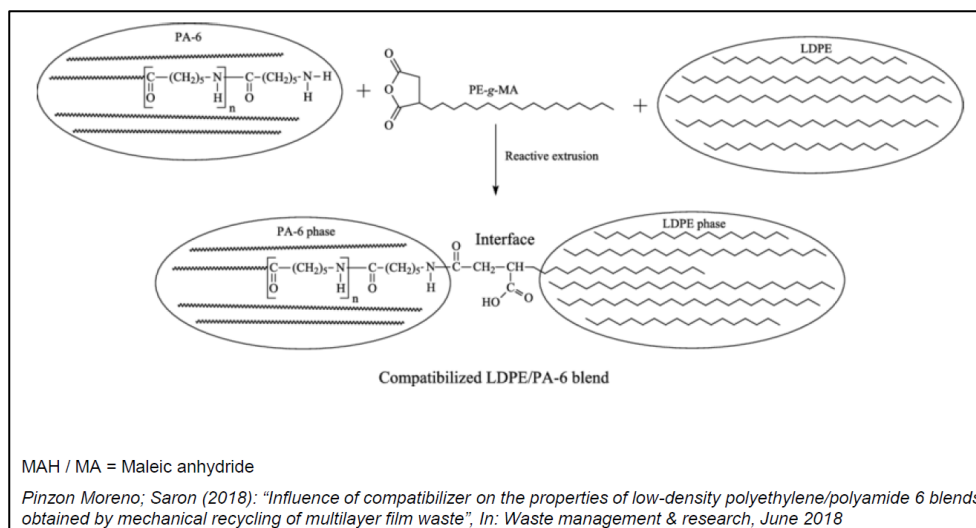
Fig. 22: Basic principle of tie layer adhesion between polyethylene and polyamide
