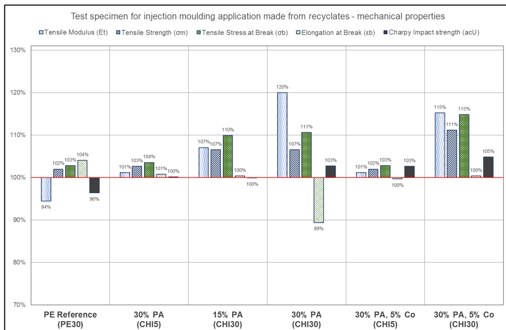
Fig. 28: Mechanical characteristic values of various recyclate samples, measured on the basis of injection molding specimens
