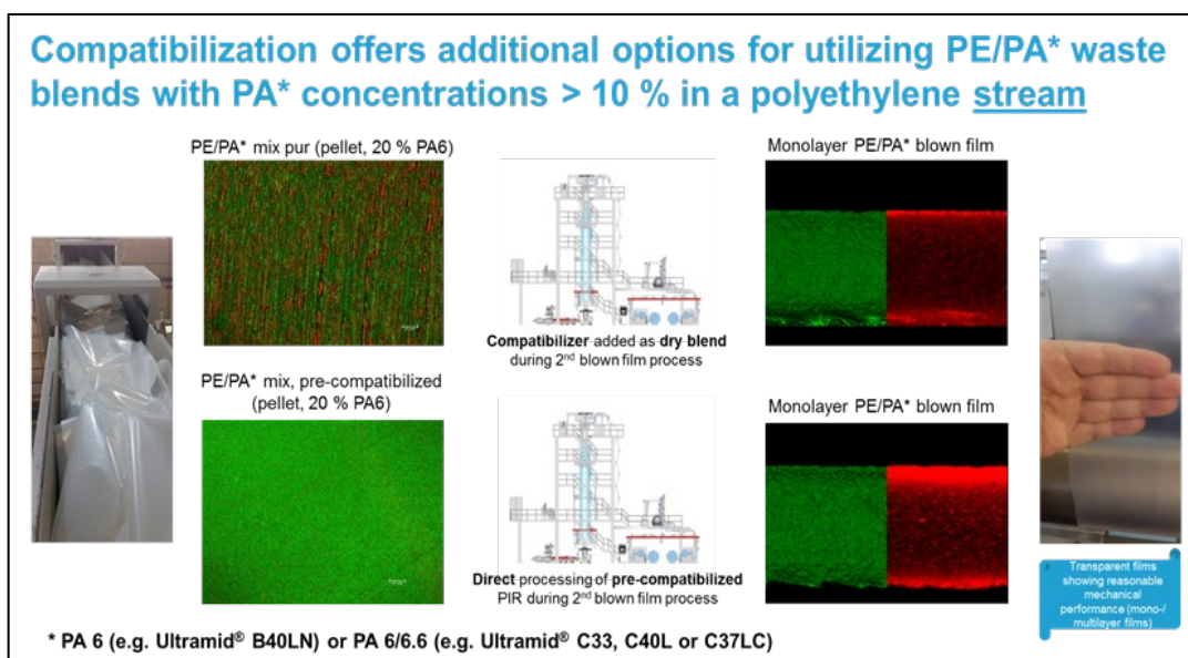
Fig. 21: Summary of process recommendation for PE/PA mixtures with >= 10 % PA
