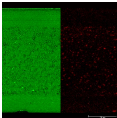
Fig. 15: Morphology of multi 3 (6.4 % PA6 in core, precompatibilized)
