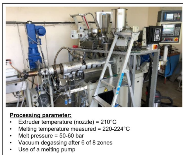
Fig. 27: Overview of extruder and processing conditions for compounding
