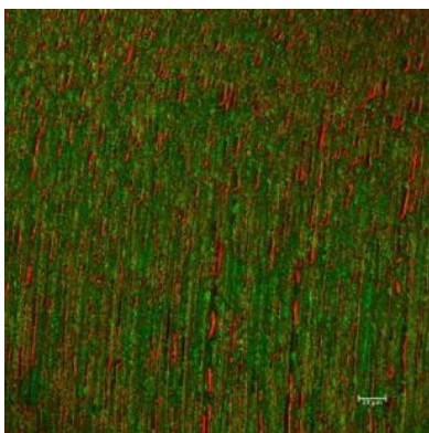
Fig. 3a: Morphology of regranulate B
