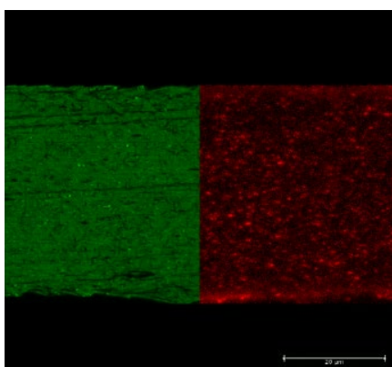
Fig. 10: Morphology of film 4.10 (contains 15 % PA6/6.6 and 3 % E226)
