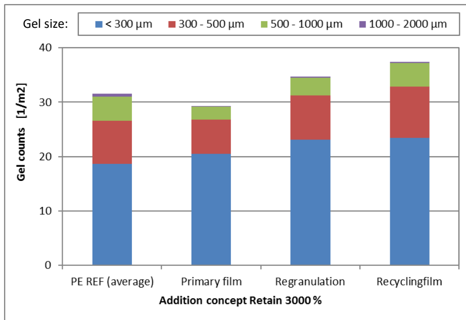
Fig. 19: Number of gels in multilayer films containing regranulate, as a function of the place of addition of Retain 3000 compatibilizer
