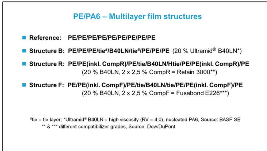
Fig. 2: Selected examples of multilayer film structures investigated
