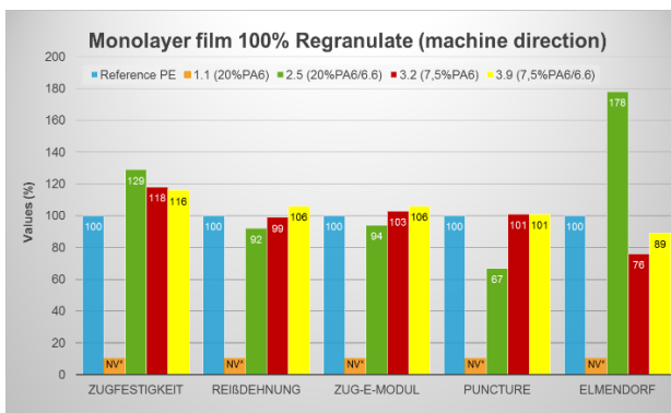
Fig. 5a: Mechanical film properties, dilution without compatibilizer (longitudinal)
