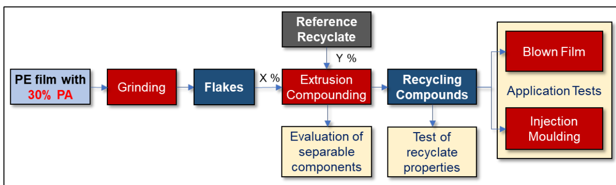
Fig. 23: Schematic diagram of the CHI standard test method CHI-C8-PEF-1
