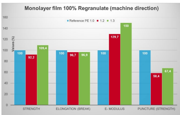
Fig. 4a: Mechanical film properties for 3 basic recipes (longitudinal)
