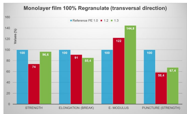
Fig. 4b: Mechanical film properties for 3 basic recipes (transversal)
