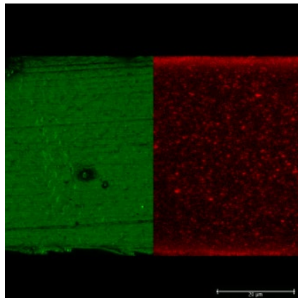
Fig. 8: Morphology of film 4.2 (contains 10 % PA6 and 5 % E226, compatibilized via premixing)
