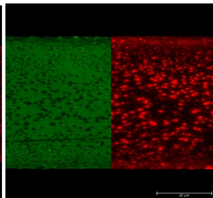
Fig. 11: Morphology of film 3.8 (contains 10 % PA6/6.6)
