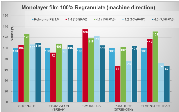
Fig. 6a: Mechanical film properties PE/PA6, dilution with added compatibilizer (longitudinal)
