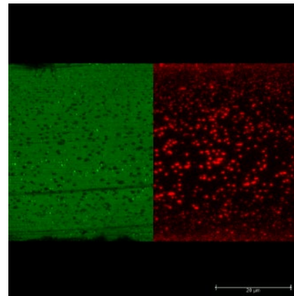
Fig. 9: Morphology of film 3.3 (contains 5 % PA6/6.6)
