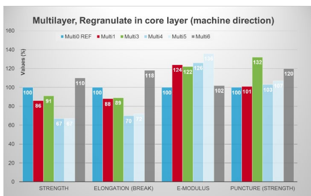
Fig. 13a: Mechanical values for multilayer films containing regranulate (longitudinal)
