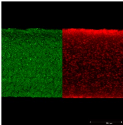
Fig.7: Morphology of film 1.2 (contains 20 % PA6 and 5 % E226, pre-compatibilized)
