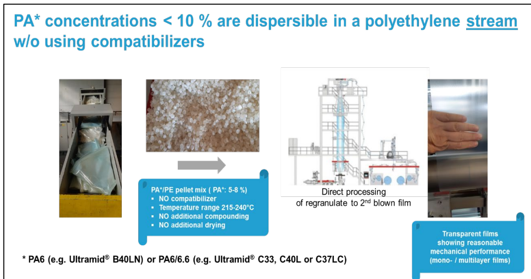
Fig. 20: Summary of process recommendation for PE/PA mixtures with < 10 % PA
