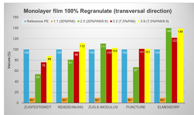
Fig. 5b: Mechanical film properties, dilution without compatibilizer (transversal)
