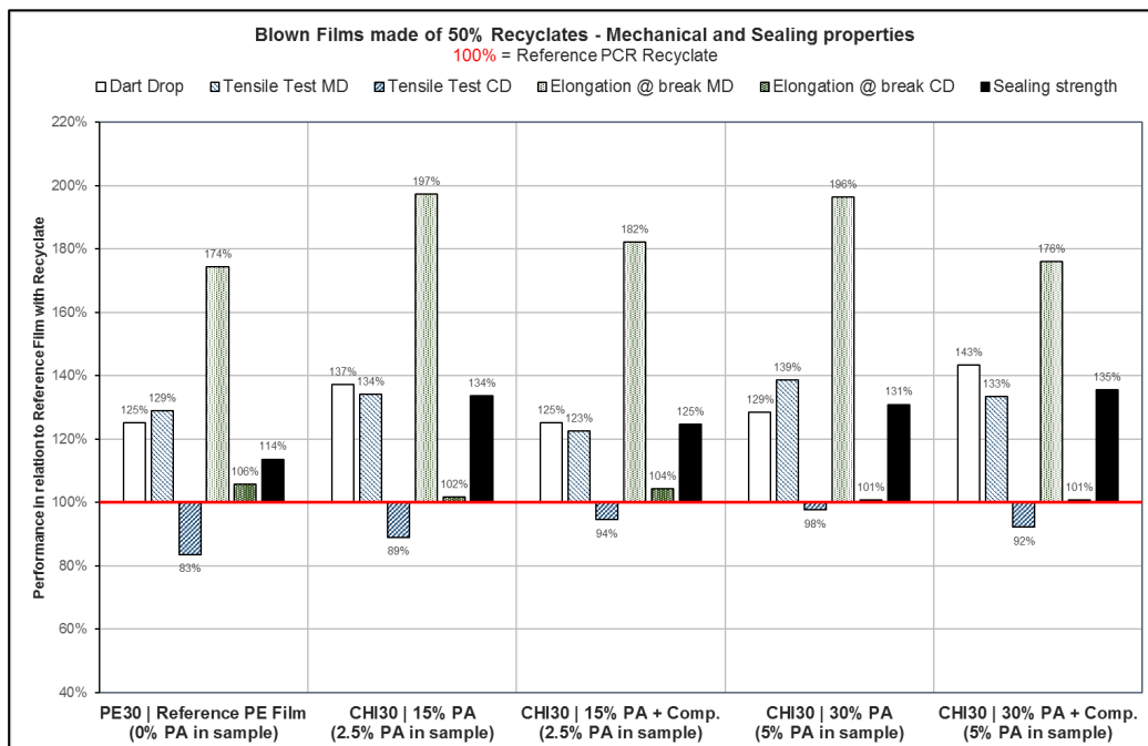
Fig. 34: Mechanical characteristic values of various recycle samples, measured on the basis of blown films
