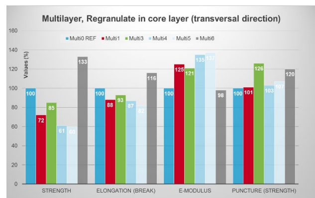
Fig. 13b: Mechanical values for multilayer films containing regranulate (transversal)
