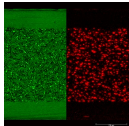
Fig. 16: Morphology of multi 5 (19.6 % PA6 in core , 2 % Retain 3000)
