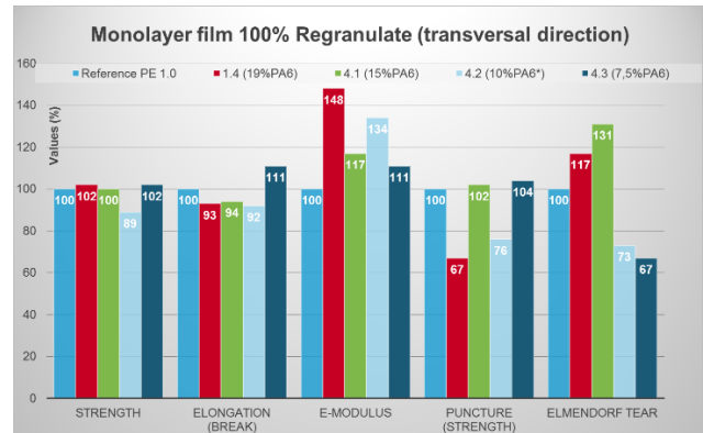
Fig. 6b: Mechanical film properties PE/PA6, dilution with added compatibilizer (transversal)
