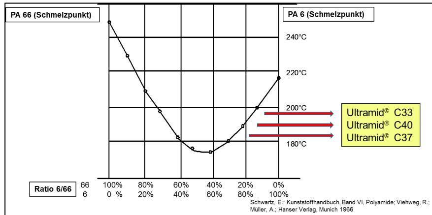
Fig. 35: Correlation of melting points of PA6/6.6 copolyamides
